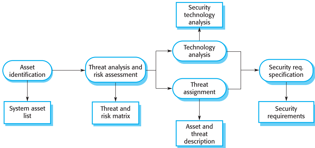
Figure 9.8 Security specification
