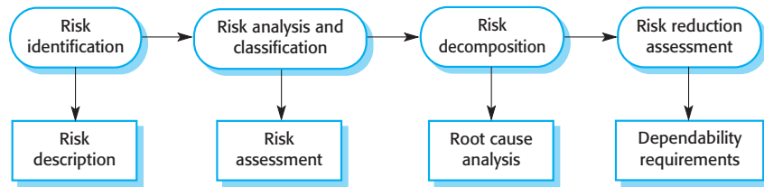
Figure 9.1 Risk-driven specification
