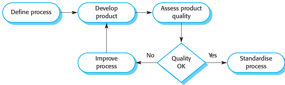
Figure 27.2 Process-based quality
